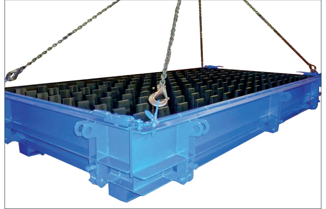
Plaque treillis
